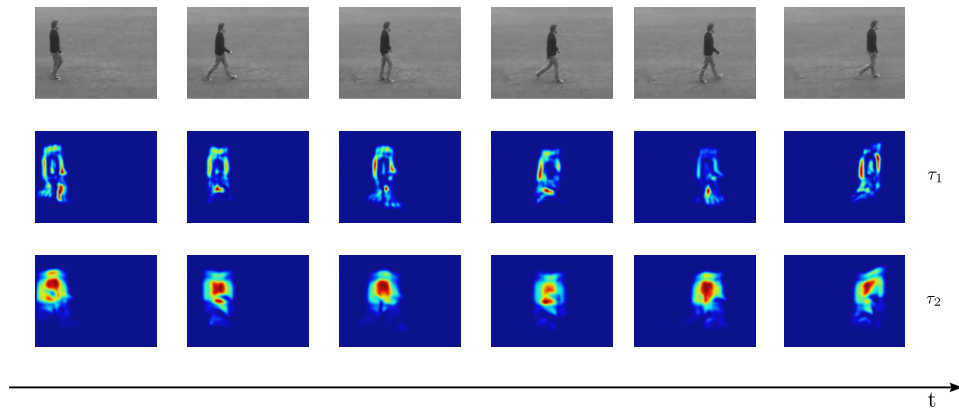
Fig. 1: Response of the spatio-temporal interest point detector at two temporal scales \tau_1 < \tau_2 (low response in blue, high response in red); first row: original video frames, second row detector response at temporal scale \tau_1 (mostly due to motion of human limbs); third row: detector response temporal scale \tau_2 (mostly due to motion of human torso).
