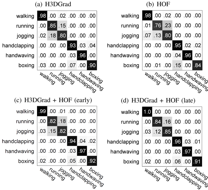
Fig. 4: Classification accuracy on the KTH dataset using k-means clustering, hard assignment and different descriptors combination strategies (i.e. early or late fusion).
