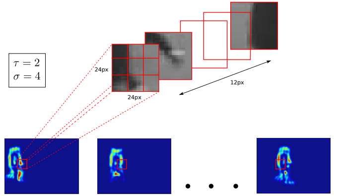
Fig. 2: Three dimensional region at the spatio-temporal interest point corresponding to a swinging arm.
