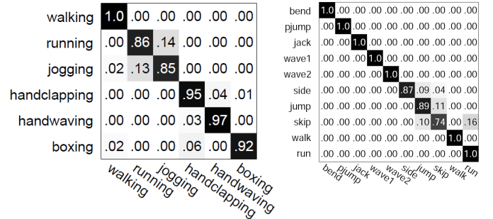
Fig. 7: Classification accuracy on KTH (left) and Weizmann (right) datasets using radius-based clustering with soft assignment.
