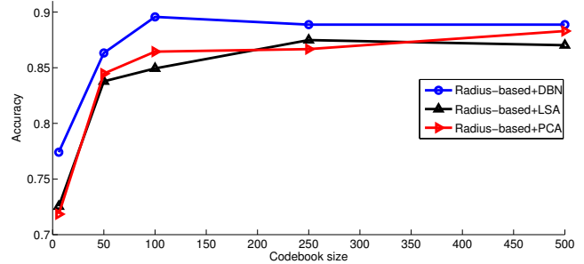
Fig. 11: Classification accuracy on KTH dataset at different codebook sizes, with different codebook reduction techniques, for radius-based clustering with soft assignment.
