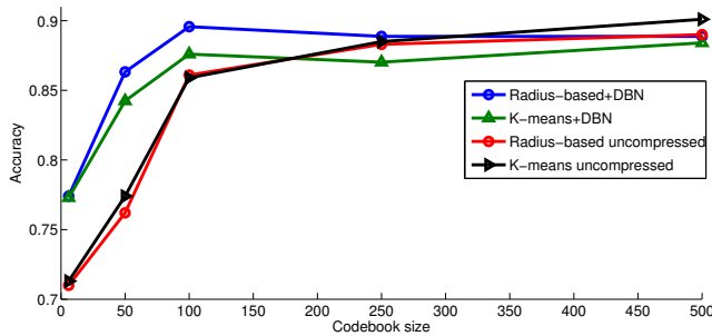
Fig. 13: Classification accuracy as a function of codebook size, for DBN-compressed and uncompressed codebooks. Radius-based clustering with soft assignment is compared with k-means clustering with hard assignment.
