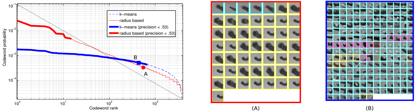
Fig. 5: Log-log plots of codeword frequency using k-means and radius-based clustering with hard assignment. Bold lines indicate regions where the average cluster precision [45] is below 0.53. The dotted diagonal line represents the Zipfian distribution. Two sample clusters are shown at near frequencies, respectively obtained with radius-based clustering (A) (most of the features in the cluster represent spatio-temporal patches of the same action) and with k-means (B) (features in the cluster represent patches of several actions). Patches of actions have different colors: boxing (cyan), hand-waving (magenta), hand-clapping (yellow), running (green), walking (red), jogging (blue).
