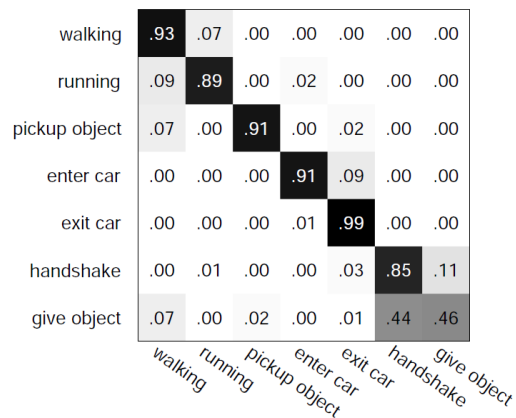
Fig. 9: Classification accuracy on the MICC-Surveillance dataset using radius-based clustering with soft assignment.
