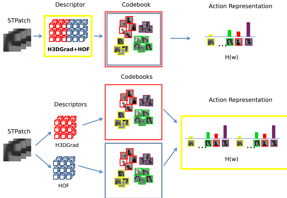
Fig. 3: Two fusion strategies: early-fusion (at the descriptor level) and late-fusion (at the codebook level).
