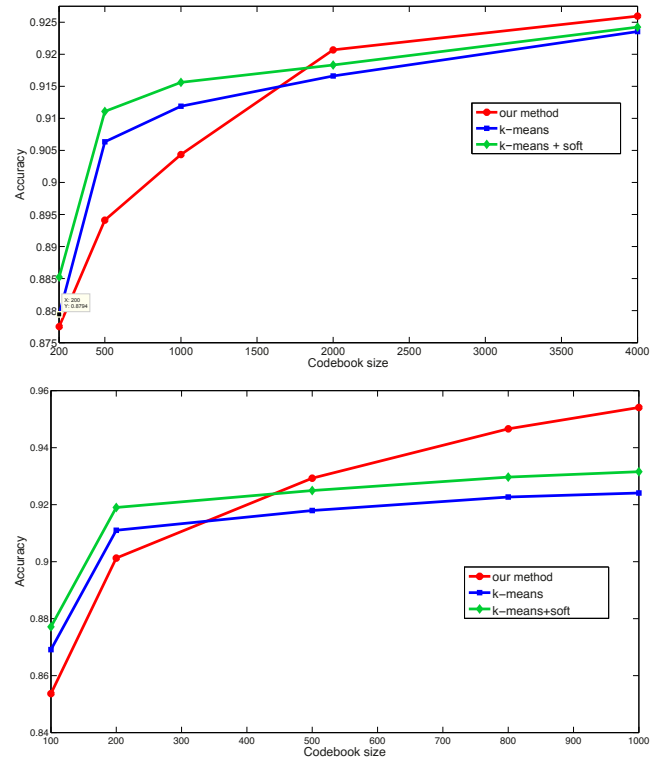
Fig. 6: Classification accuracy on KTH (top) and Weizmann (bottom) datasets with codebooks created with k-means with hard assignment, k-means with soft assignment and radius-based with soft assignment.
