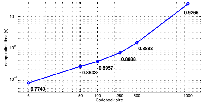
Fig. 12: Mean computation times for a KTH video sequence at different codebook sizes with radius-based clustering and DBNs. The numbers associated to the markers indicate the classification accuracy.
